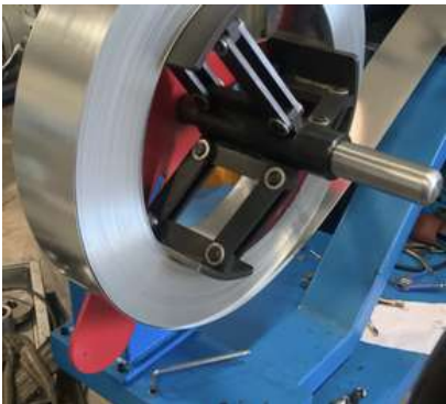
Proses Rolling
